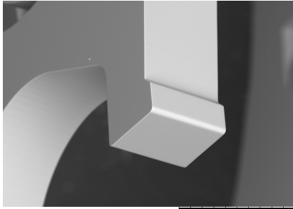
Detail of escape-wheel
